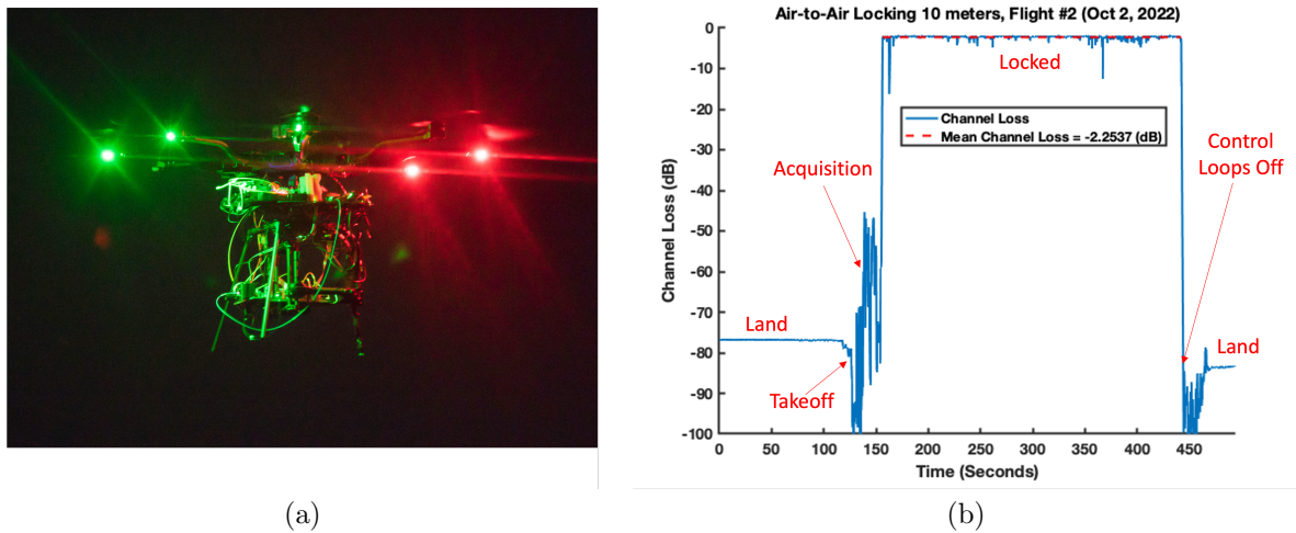
Figure 3. Air-to-Air Classical Locking. (a). Air-to-Air Setup, (b) Classical Channel Loss vs Time into multimode fiber.
