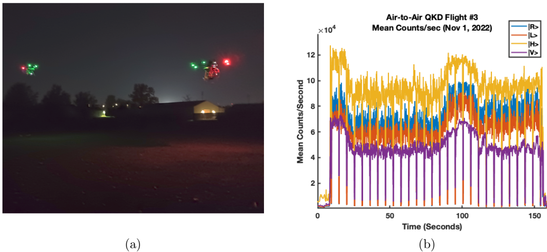
Figure 4. Air-to-air drone-based QKD. (a). Air-to-air setup, and (b) temporal evolution of the QKD transmission (1-sec integration time).
